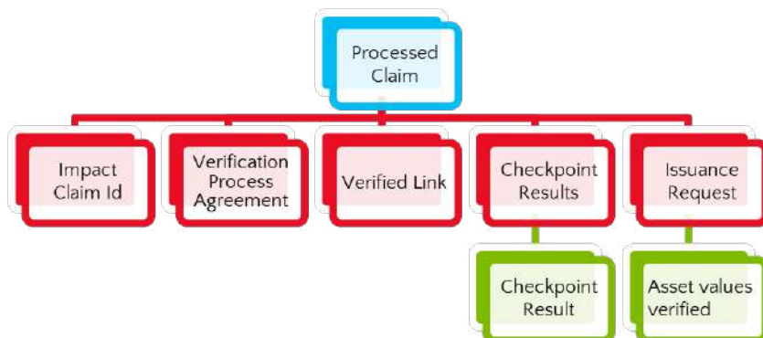
Figure 5: Processed Claim
